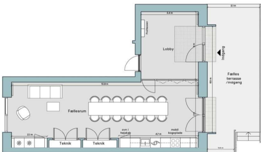
stue
