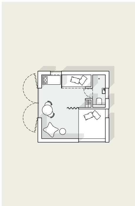
Plan 1: 150
